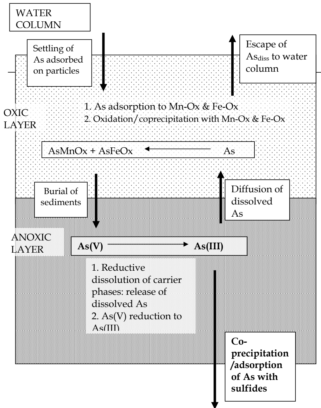
Figure 2: Conceptual Model of Early Arsenic Diagenesis. Arrows indicate fluxes and transport of arsenic (Figure adapted from Edenborn et al. (1986), Belzile (1988), Wilderlund and Ingri (1995), Sullivan and Aller (1996) Mucci et al (2000)).
